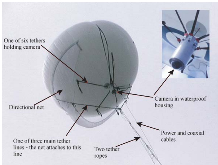
The “blimp-cam”, consisting of the new ovoid style blimp and off-the-shelf dome security camera within a custom made waterproof housing.
