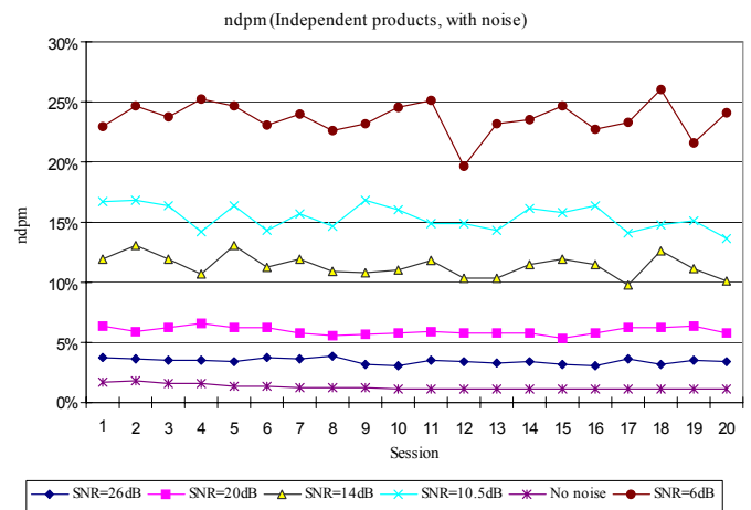
Fig. 6. The ndpm on Independent Products With Noise
