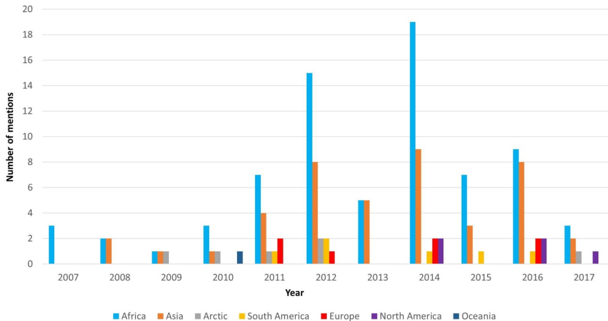
Figure 1: Frequency of mentions of continents in the climate-conflict literature per year
