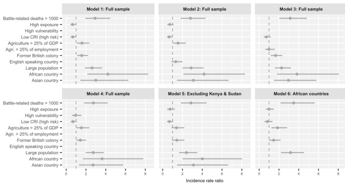
Figure 2: Changes in the frequency of mentions in the climate-conflict literature depending on country characteristics
