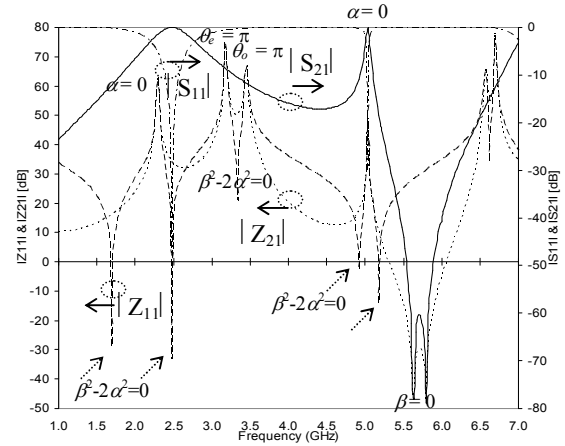
Figure 5: |Z_{11}| , |Z_{21}| , |S_{11}| and |S_{21}| of simple single-stage PCMBF with w=1\text{mm} , s=0.2\text{mm} and l=14.6\text{mm} .
