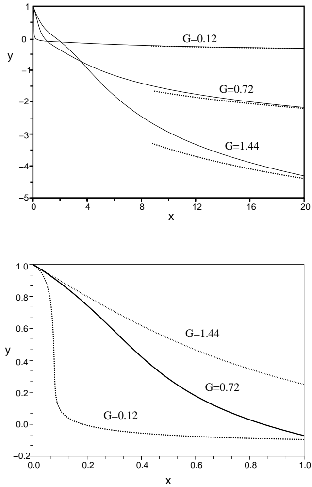
Figure 3. (a) Interface shapes with \alpha = -\pi/4 , for G = 0.12, 0.72 and 1.44 compared with the asymptotic solution given by (22). (b) close-up view of the same showing behaviour near to the sink. Note the steepening of the surface as the nondimensional flow rate, G , decreases.
