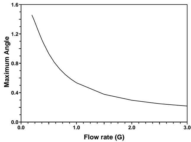
Figure 6. Maximum slope on the interface near to (but not at) the sink as a function of flow rate for the special solution branch where entry angle into the line sink was zero, \alpha = 0 . As G decreases the steepest angle approaches vertical as G approaches 0.12.
