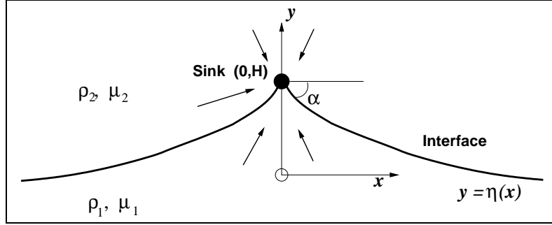
Figure 1. Schematic of the flow into a line sink from two layers of different density - supercritical flow rate.
