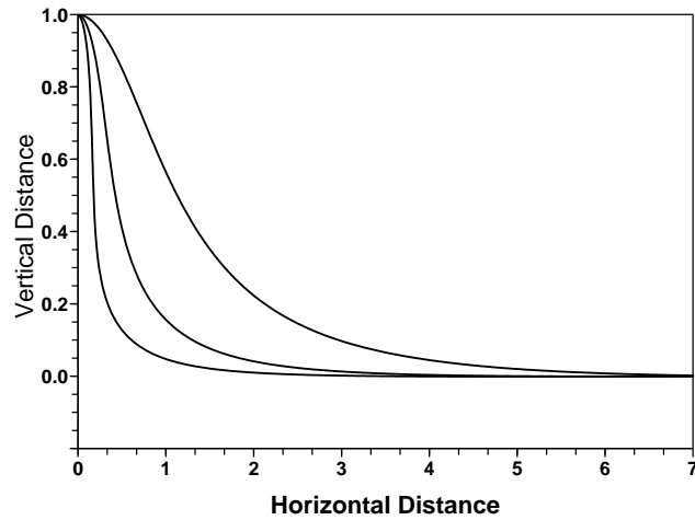
Figure 5. Interface shapes for the special case with \alpha = 0 and G = 0.16, 0.24 and 0.81 (from left to right respectively) for the unbounded two-layer flow where the interface levels off at y = 0 .
