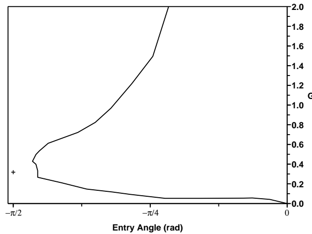
Figure 4. Solution domain showing angle of entry against G . Solutions exist everywhere to the right of the given curve. The lower limit is characterised by the interface slope becoming very steep near to the sink, as in Figure 3(b), G = 0.12 . The + is the solution of [2] for critical single layer flow.
