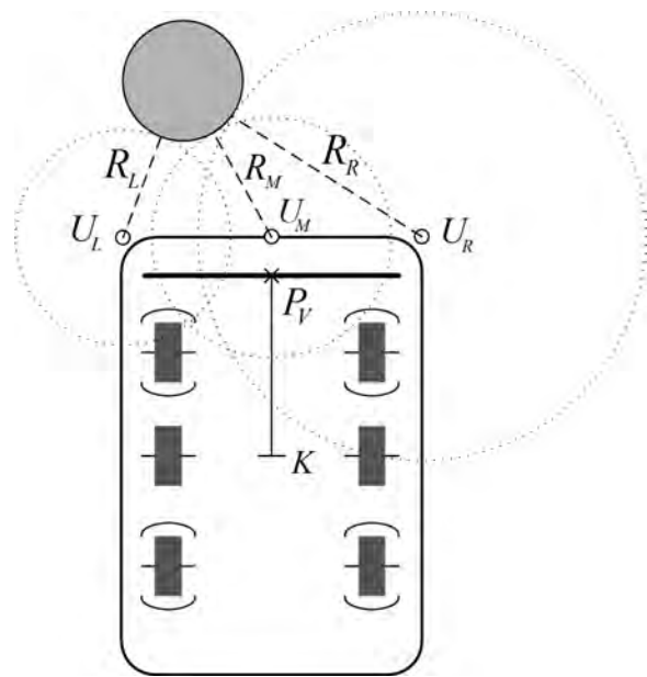
Fig. 2. Obstacle sensor.
