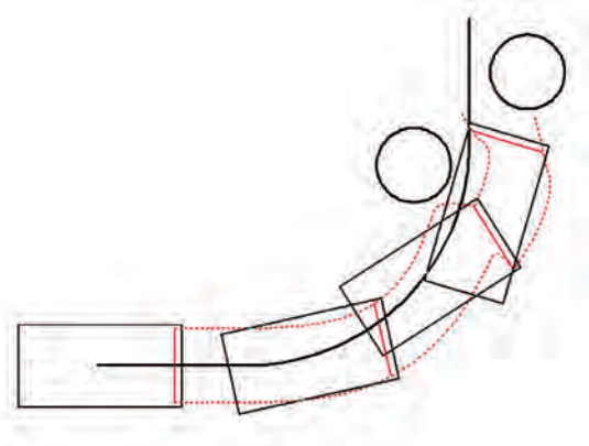
Fig. 14. Result by Controller A.
