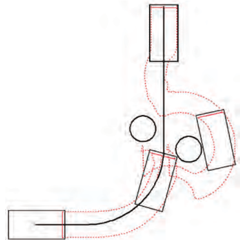
Fig. 13. Reverse strategy by adjusting original FRI.
