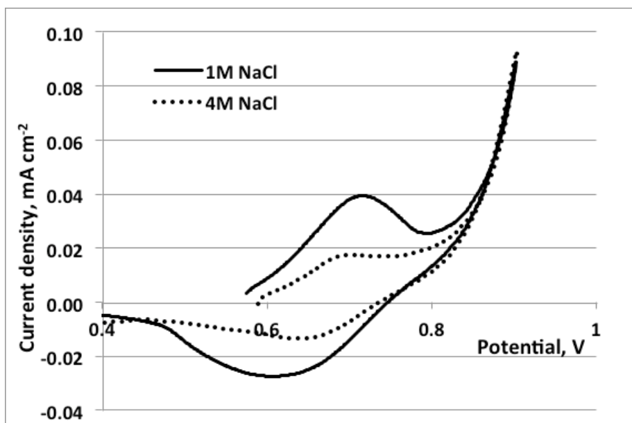
Fig. 9 Cyclic voltammograms (1 mV/s) for the anodic oxidation of a rotating (200rev/min) pyrite electrode in solutions of 1M and 4M NaCl with 0.02M HCl at 25°C. These results agree with published data that showed no effect of chloride between 0.25M and 1.0M (Bryson and Crundwell, 2014) at potentials up to 1.4V.
