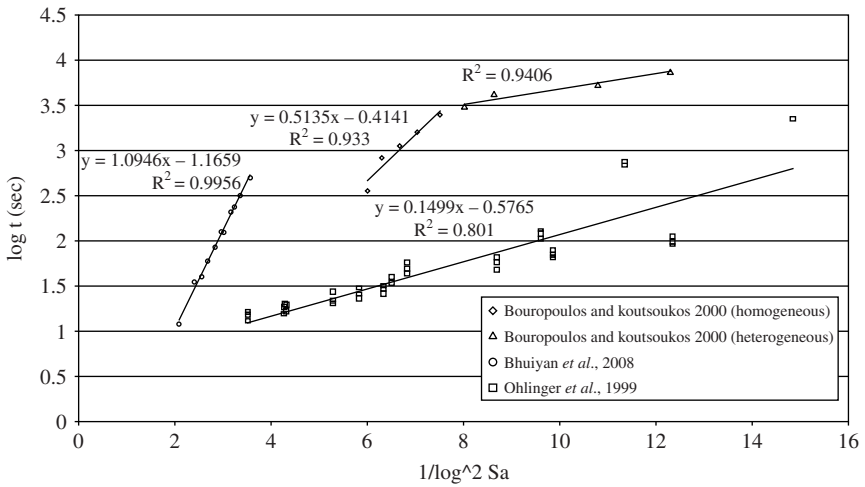
Figure 3. Logarithmic plots of induction time versus the inversed square of supersaturation ratio for the previous studies.
