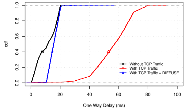
Fig. 8. CDF of one way delay for game flow on a 15 Mbps link. Measured in the client to server direction.
