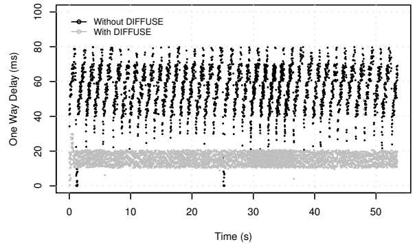
Fig. 9. With and without DIFFUSE: per-packet one way delay for game flow with TCP cross traffic on a 15 Mbps link. Measured in the client to server direction
