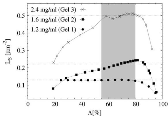
FIGURE 9 Specific length, i.e., length/volume, of the collagen fiber network as function of segmentation parameter \Lambda .
