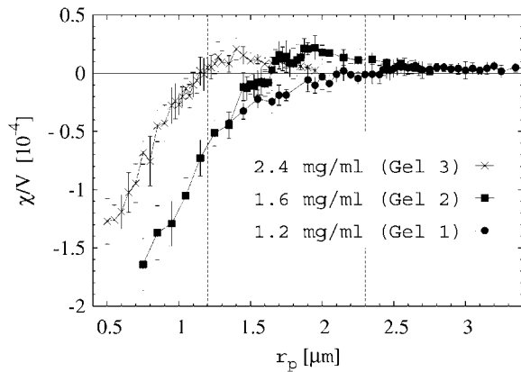
FIGURE 10 The Euler index of diluted versions of the collagen network as a function of the dilation radius. The vertical lines mark the dilation radius D_\chi for which \chi vanishes.
