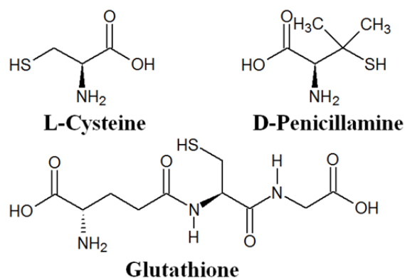
Fig. 1 Structural formulas of the thioamino acids CSH, PSH and GSH.
