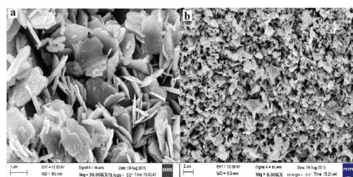
Fig. 3: FESEM images of \text{Co}(\text{OH})_2
