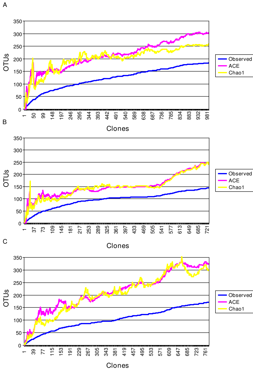
Figure 2 Collector's curves of the observed and estimated phylotype richness of 16S rRNA gene libraries. Collector's curves of the observed (blue) and estimated (ACE (pink) and Chao1 (yellow)) phylotype richness calculated for IN (A), OUT (B) and IR (C) at 99% level. Each curve reflects observed or estimated richness values obtained as more clones are added to the data set. After an initial steep rise, the curves level out suggesting that a majority of clones in the treatment groups have been sampled. Differences between the estimates and observed phylotype richness were highest in the IR group. Novel phylotypes continued to be identified up to the end of sampling in this group.
