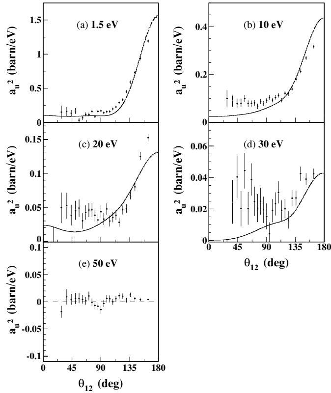
Figure 2. |a_u|^2 at E_{\text{exc}} = 100 eV on absolute scale. The solid line is the velocity form of a CCC calculation. Energy integration of one of both electrons: (a) 0 < E_e < 3 eV, (b) 5 < E_e < 15 eV, (c) 15 < E_e < 25 eV, (d) 25 < E_e < 35 eV, (e) 45 < E_e < 55 eV. To guide the eye, a dashed line is drawn at |a_u|^2 = 0 in panel (e).
