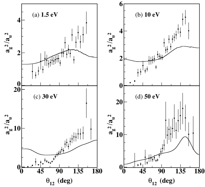
Figure 7. |a_g|^2/|a_u|^2 at E_{\text{exc}} = 450 eV. The solid line is the velocity form of a CCC calculation. Energy integration of one of both electrons: (a) 0 < E_e < 3 eV, (b) 5 < E_e < 15 eV, (c) 25 < E_e < 35 eV, (d) 45 < E_e < 55 eV.
