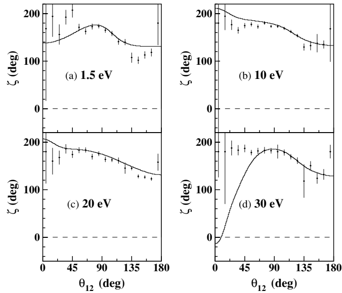
Figure 4. Phase between a_g and a_u at E_{\text{exc}} = 100 eV. The whole COLTRIMS data set for linearly and circularly polarized light is used. The phase \zeta is given by \sin \zeta = \text{CD}/(-4 \sin \Phi_{12} |a_g| |a_u|) . The solid line is the velocity form of a CCC calculation. Energy integration of one of both electrons for linearly and circularly polarized light: (a) 0 < E_e < 3 eV, (b) 5 < E_e < 15 eV, (c) 15 < E_e < 25 eV, (d) 25 < E_e < 35 eV, (e) 45 < E_e < 55 eV. For circularly polarized light, the two electrons are in a plane perpendicular to the light propagation: \Theta_1 = \Theta_2 = 90^\circ \pm 7^\circ . To guide the eye a dashed line is drawn at \zeta = 0^\circ .
