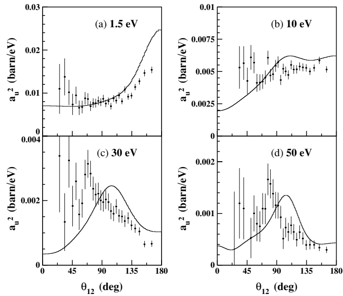
Figure 6. |a_u|^2 at E_{\text{exc}} = 450 eV. The data set is normalized to the CCC calculation. The whole COLTRIMS data set for linearly polarized light is used for extracting |a_u|^2 . The solid line is the velocity form of a CCC calculation. Energy integration of one of both electrons: (a) 0 < E_e < 3 eV, (b) 5 < E_e < 15 eV, (c) 25 < E_e < 35 eV, (d) 45 < E_e < 55 eV.
