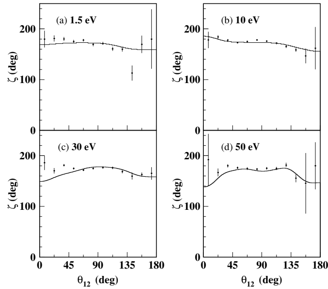
Figure 8. Phase between |a_g| and |a_u| at E_{\text{exc}} = 450 eV. The whole COLTRIMS data set for linearly and circularly polarized light is used. The phase \zeta is given by \sin \zeta = \text{CD}/(-4 \sin \Phi_{12} |a_g| |a_u|) . The solid line is the velocity form of a CCC calculation. Energy integration of one of both electrons for linearly and circularly polarized light: (a) 0 < E_e < 3 eV, (b) 5 < E_e < 15 eV, (c) 25 < E_e < 35 eV, (d) 45 < E_e < 55 eV. For circularly polarized light, the two electrons are in a plane perpendicular to the light propagation: \Theta_1 = \Theta_2 = 90^\circ \pm 25^\circ .
