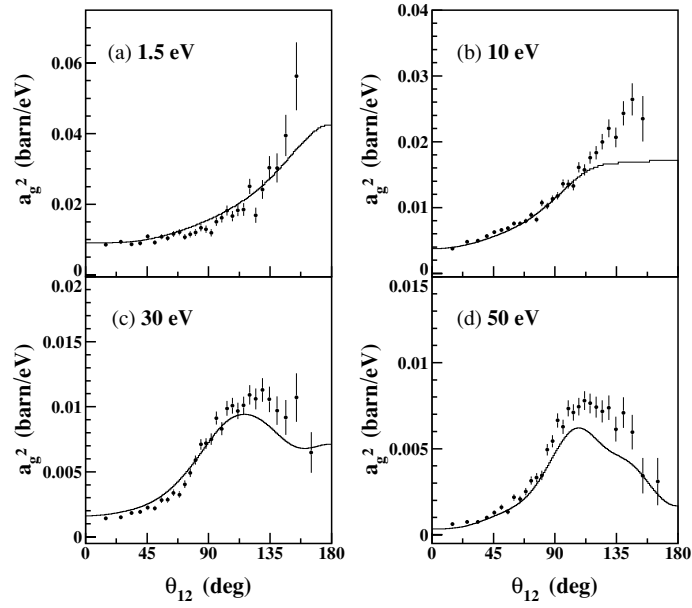
Figure 5. |a_g|^2 at E_{\text{exc}} = 450 eV. The data set is normalized to the CCC calculation. The whole COLTRIMS data set for linearly polarized light is used for extracting |a_g|^2 . The solid line is the velocity form of a CCC calculation. Energy integration of one of both electrons: (a) 0 < E_e < 3 eV, (b) 5 < E_e < 15 eV, (c) 25 < E_e < 35 eV, (d) 45 < E_e < 55 eV.
