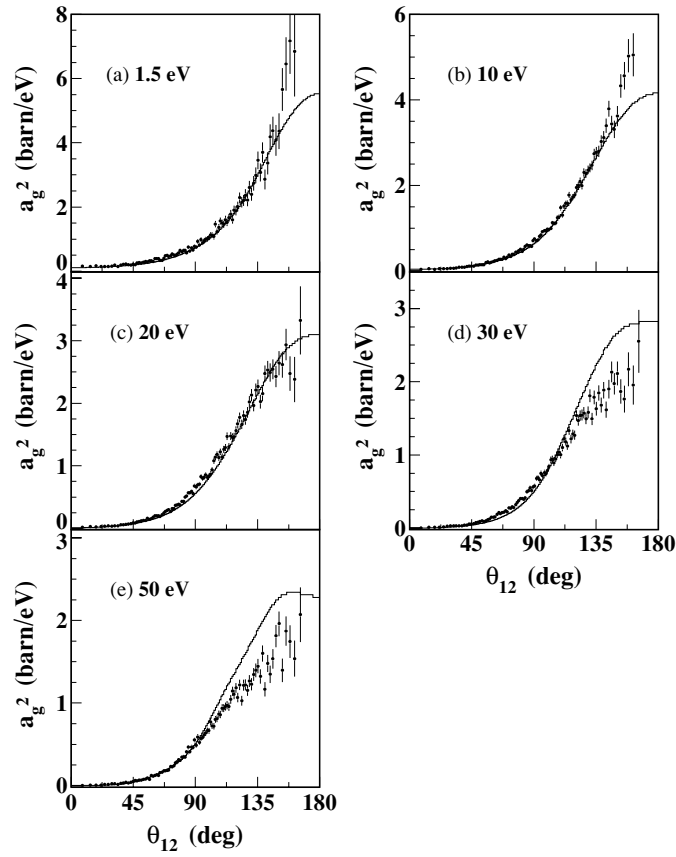
Figure 1. |a_g|^2 at E_{\text{exc}} = 100 eV on absolute scale. The whole COLTRIMS data set for linearly polarized light is used for extracting |a_g|^2 . The solid line is the velocity form of a CCC calculation. Energy integration of one of both electrons: (a) 0 < E_e < 3 eV, (b) 5 < E_e < 15 eV, (c) 15 < E_e < 25 eV, (d) 25 < E_e < 35 eV, (e) 45 < E_e < 55 eV.
