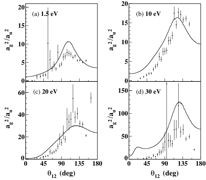
Figure 3. |a_g|^2/|a_u|^2 at E_{\text{exc}} = 100 eV. The solid line is the velocity form of a CCC calculation. Energy integration of one of both electrons: (a) 0 < E_e < 3 eV, (b) 5 < E_e < 15 eV, (c) 15 < E_e < 25 eV, (d) 25 < E_e < 35 eV, (e) 45 < E_e < 55 eV.
