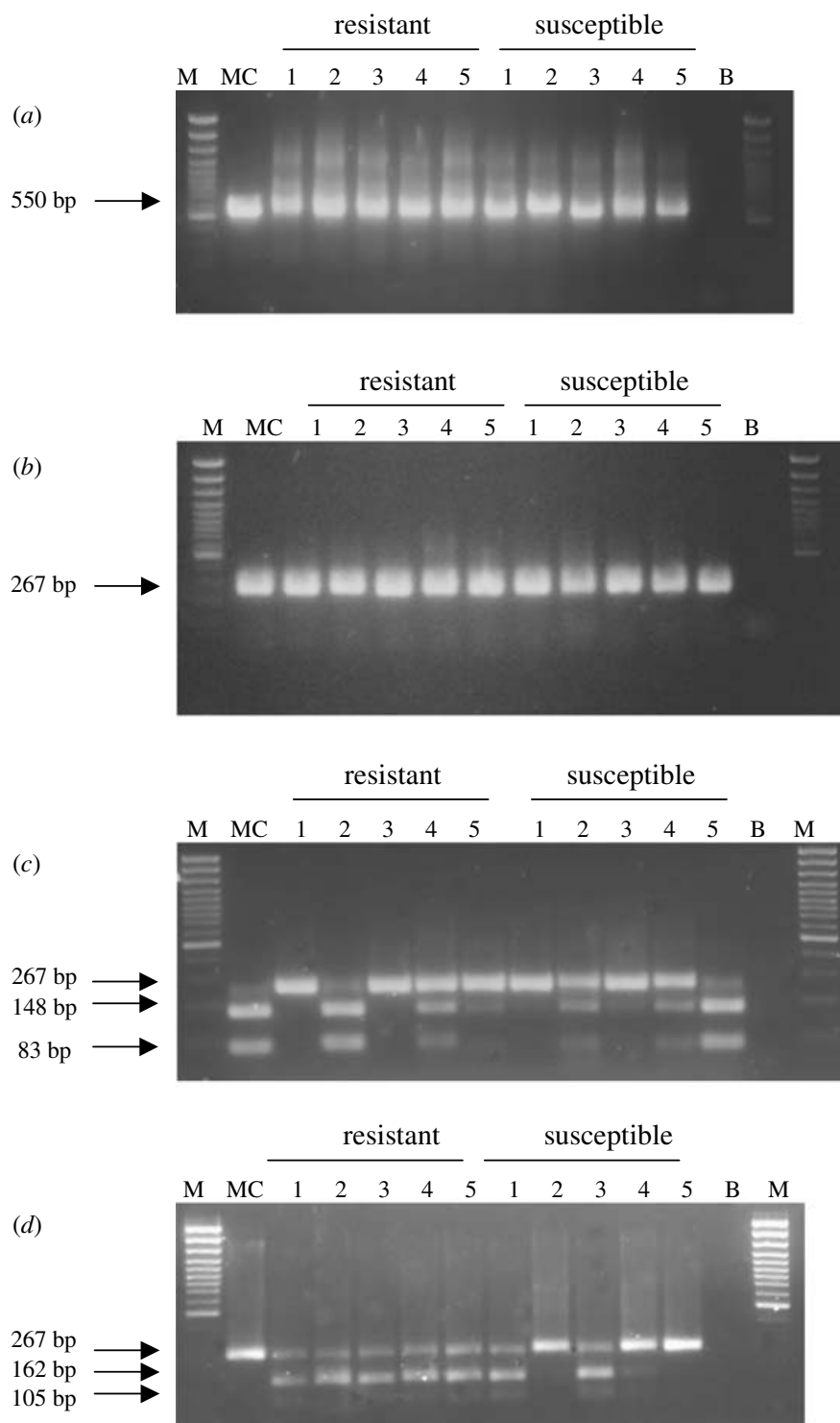
Fig. 12. PCR products of DNA from lesions on adult leaves of Eucalyptus globulus trees resistant or susceptible to Mycosphaerella leaf disease in the seed orchard with ITS1F/ITS4 (a) and MCF/MCR (b) primers and the subsequent restriction digestions of the MCF/MCR primer PCR products with Dde I (c) and Tru 1I (d). Lanes: M, 100 bp DNA ladder; MC, genomic DNA of M. cryptica (positive control); 1–5, DNA of single leaf lesions; and B, negative control.
