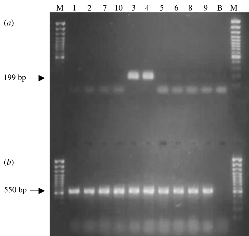
Fig. 1. PCR amplified DNA of Mycosphaerella isolates from the seed orchard with MNF/MNR ( a ) and ITS1/ITS4 ( b ) primers. Lane numbers refer to isolate numbers as indicated in Table 1. Lanes M, 100 bp DNA ladder; 1–2, 7, 10, M. cryptica ; 3–4, M. nubilosa ; 5, Mycosphaerella sp. 1; 6, Mycosphaerella sp. 2; 8–9, Mycosphaerella spp.; and B, negative control.
