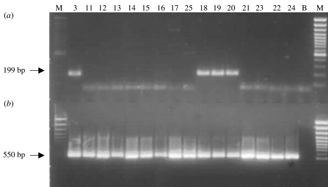
Fig. 2. PCR amplified DNA of Mycosphaerella isolates from Eucalyptus species at various locations in Victoria, Australia with MNF/MNR ( a ) and ITS1/ITS4 ( b ) primers. Lane numbers refer to isolate numbers as indicated in Table 1. Lanes: M, 100 bp DNA ladder; 3, M. nubilosa (positive control); 11, 13–17, 25, M. cryptica ; 18, M. nubilosa ; 19–20, unidentified Mycosphaerella spp. (from adult E. globulus leaves); 21, M. tasmaniensis ; 12 & 23, M. vespa ; 22 & 24, unidentified Mycosphaerella spp.; and B, negative control.
