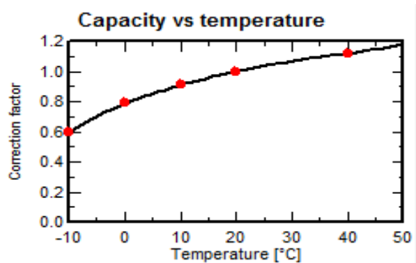
Fig. 9. Sonnenschein, A600, 1200Ah capacity at C_{10} solar battery Ah capacity correction factor versus the discharge temperature in °C.
